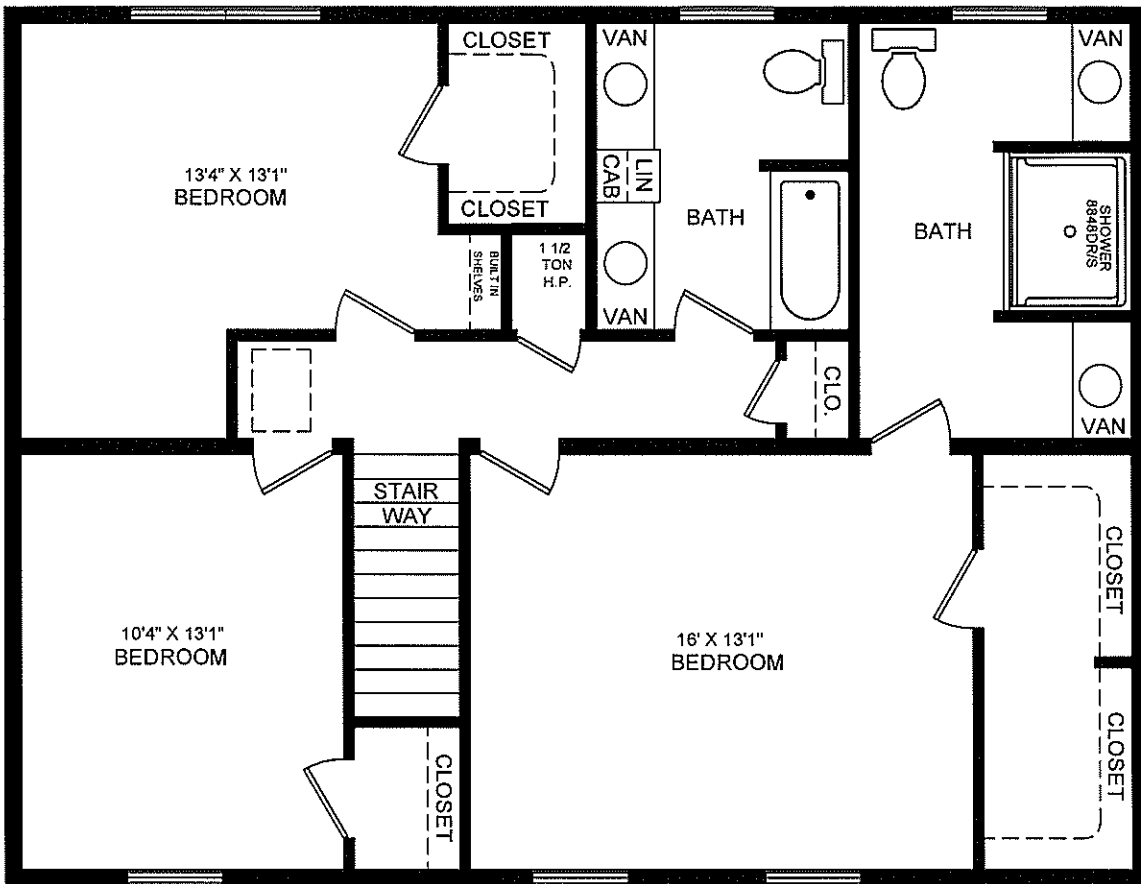
2nd FLOOR
