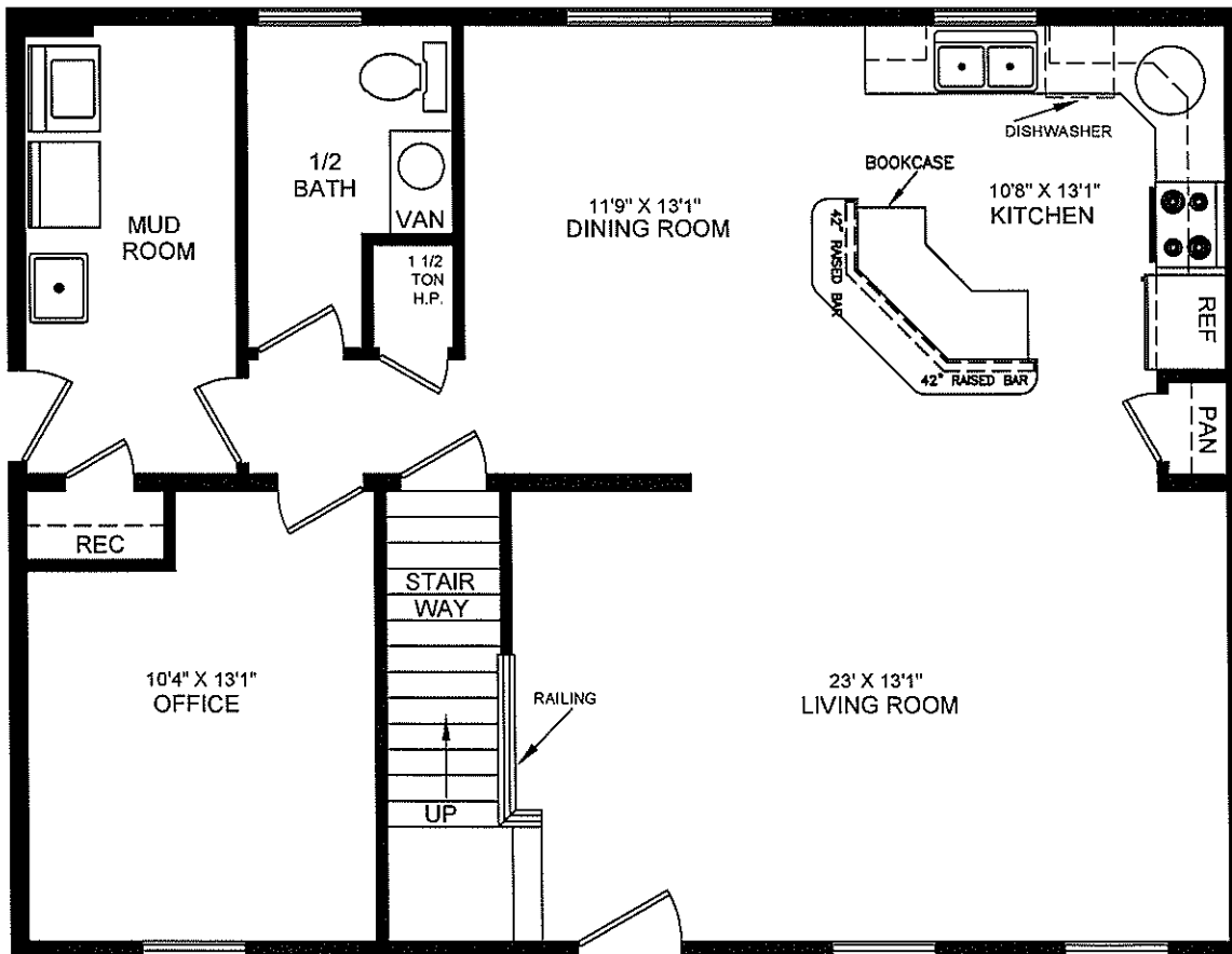
1st FLOOR
